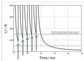
Fig. 1: Heat accumulation of single laser pulses
