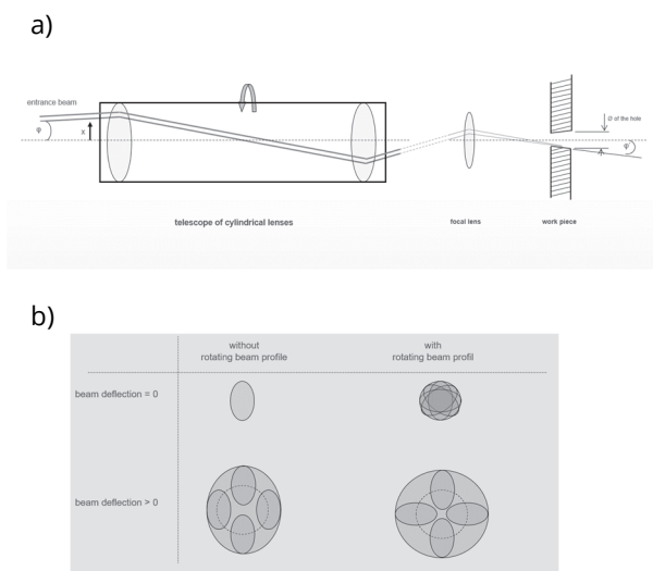
Fig. 4. (a) Optical concept of GL.trepan using a telescope of cylindrical lenses; (b) Rotation of beam profile allows drilling round holes even with elliptical beam profile
