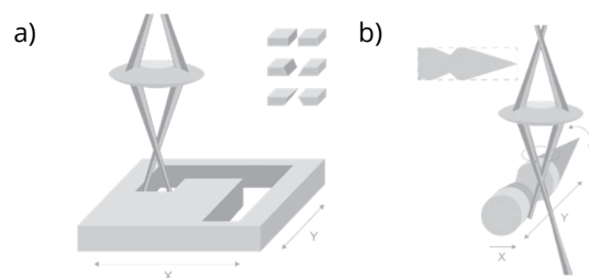
Fig. 3. (a) Precision cutting by turning tilted laser beam and moving workpiece (schematic); (b) Laser turning by rotating and tilting beam as well as linear moving and rotating workpiece (schematic)
