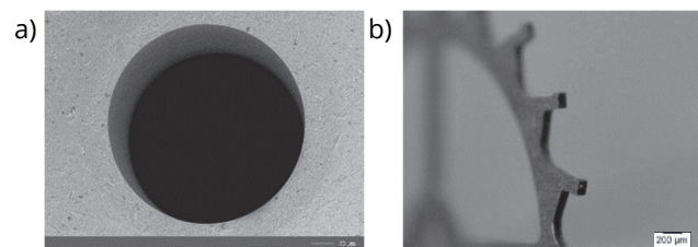
Fig. 6. (a) Micro drilling with diameter 300μm in tooling steel with thickness 200μm; Processing time: 1.7s; (b)Vertical cut of a driving wheel in brass with thickness 0.15mm for mechanical watches industries
