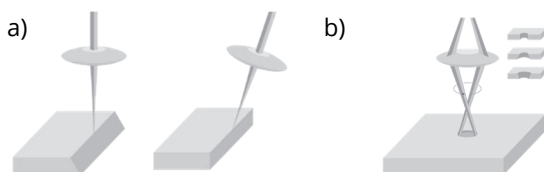
Fig. 2: (a) Influence of inclination angle on wall angle (schematic); (b) Tilted rotating laser beam allows drilling with positive and negative wall angle as well as cylindrical holes (schematic)
