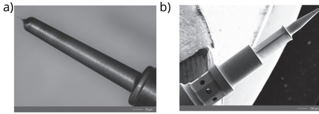
Fig. 7. (a) Laser turned ejector with a length of 9mm and end piece diameter of 40µm made of carbide; (b) Combination of laser turning, drilling and cutting processes with one clamping operation
